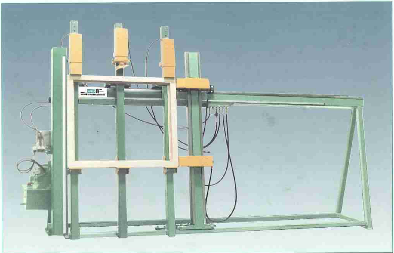
Frame Press Euro Universal with additional central pressure beam
